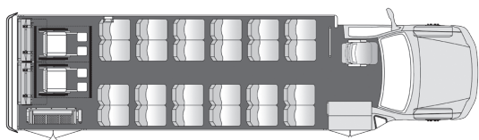
24 Passenger 2 Wheelchair with Flip Seats Plus Driver
