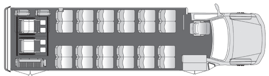
24 Passenger 2 Wheelchair with Foldaway Seats Plus Driver
