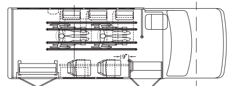
6 + 2 Passenger & 2 W/C
