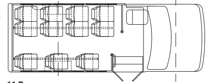
11 Passenger
