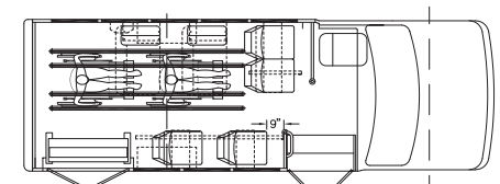
4 + 4 Passenger & 2 W/C
