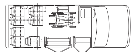
7 + 2 Passenger & 1 W/C
