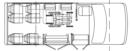
6 + 4 Passenger & 2 W/C
