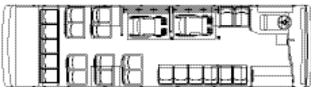
23-Passenger w/Two Wheelchairs or 29-Passenger
