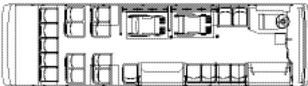
20-Passenger w/Two Wheelchairs or 26-Passenger
